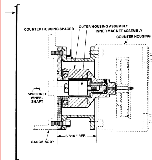
Magnetic Drive Motor Option
